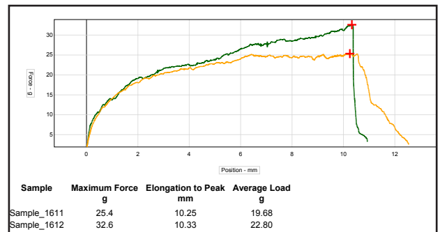
Sample test results for the Film Blocking
