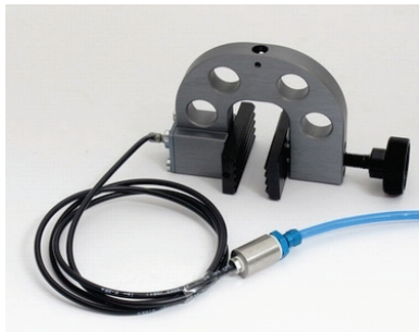
TA94 with TA94-BW50 jaws + TA205-PK23 adapter
